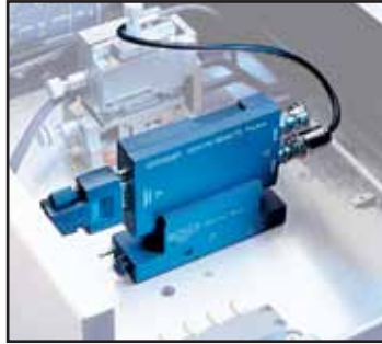
DC PreAmps can be mounted on the probe station with either a platen base or a triax mounting bracket. By reducing the signal path between the DUT and the PreAmp from several feet to a fraction of an inch, the Model 4200-SCS can eliminate cable effects like parasitic capacitance and leakage currents, which provides more accurate low-level measurements.
