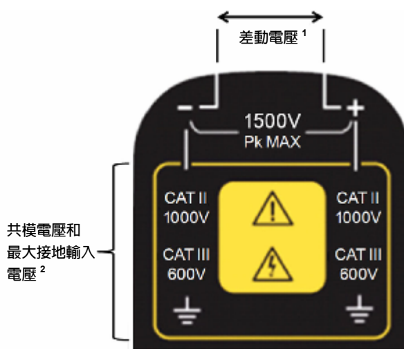
THDP0200 探棒標籤
